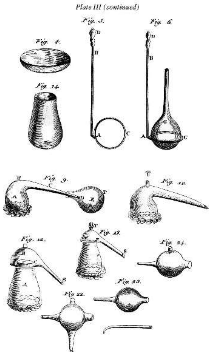
Figure 11.8: Apparatus used by Lavoisier in his chemical experiments.
